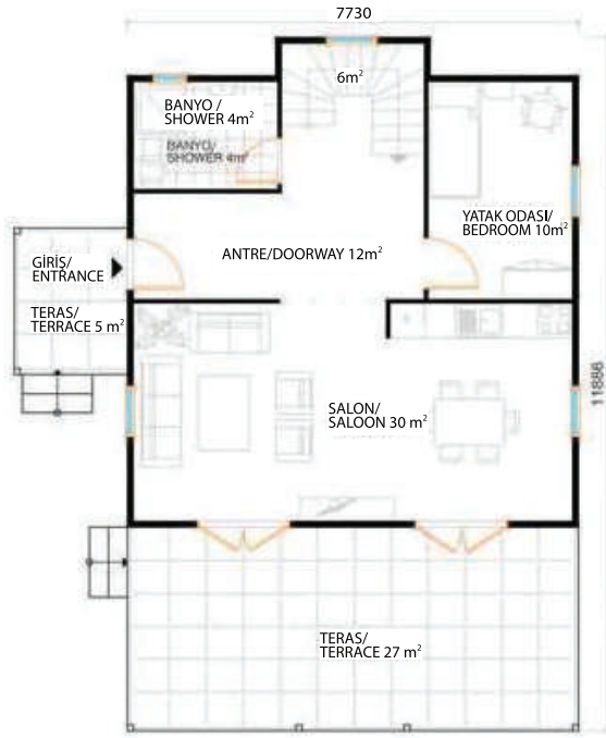
Zemin Kat Planı / Ground Floor Plan 94 m 2
